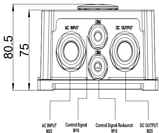
Wire Ports
