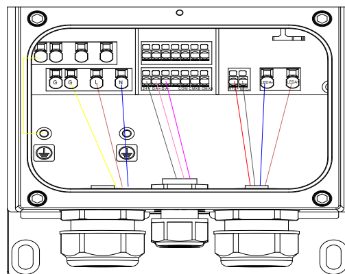
DALI&amp;DMX Wiring Connection
