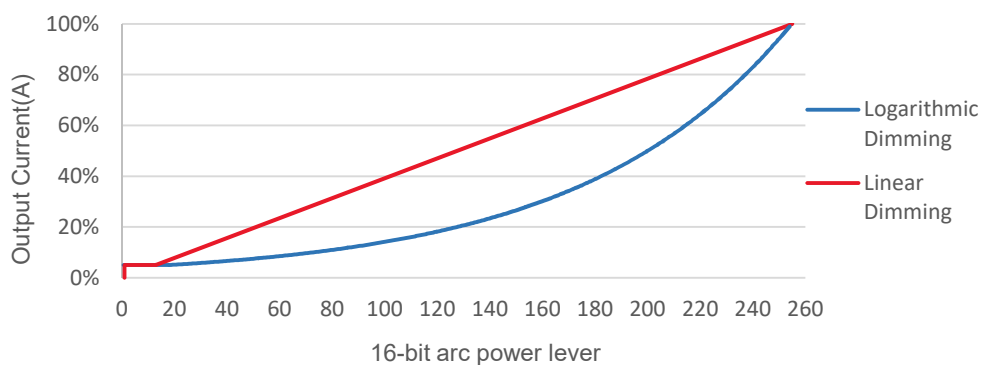
DALI-2 dimming curve
