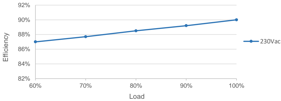
Efficiency vs. Load (I o =1.05A)
