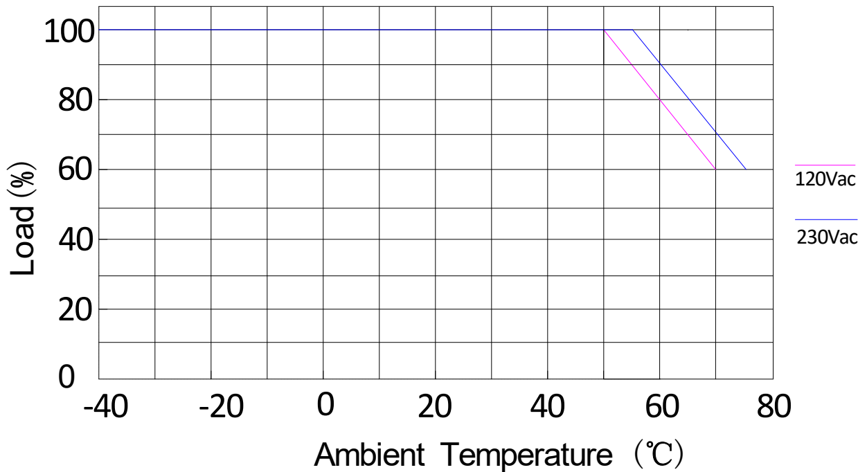
Derating Curve
