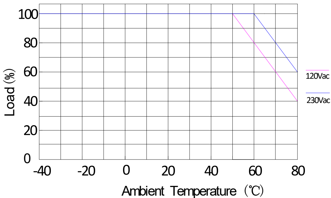
Derating Curve
