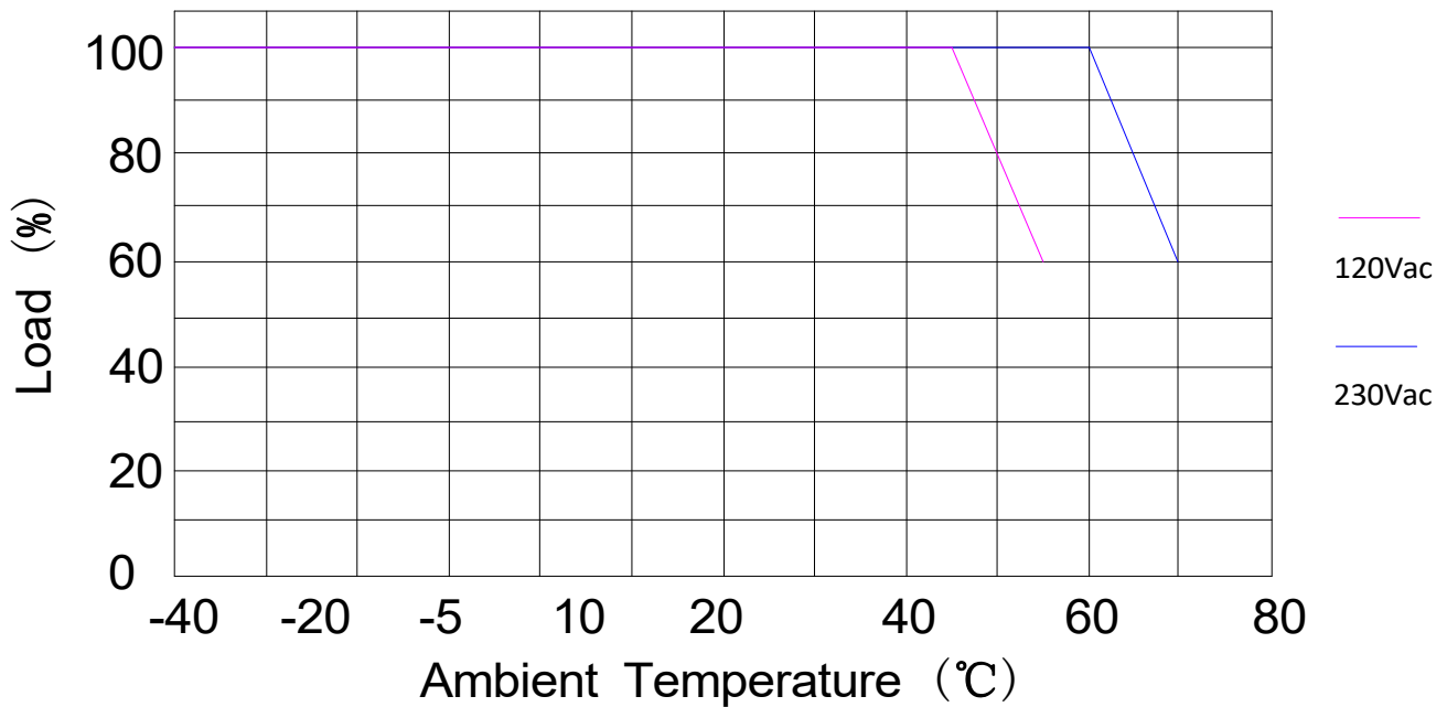
Derating Curve
