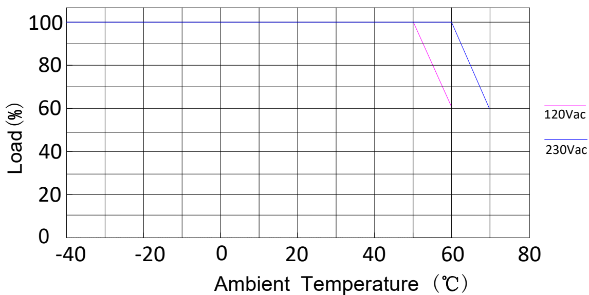
Derating Curve
