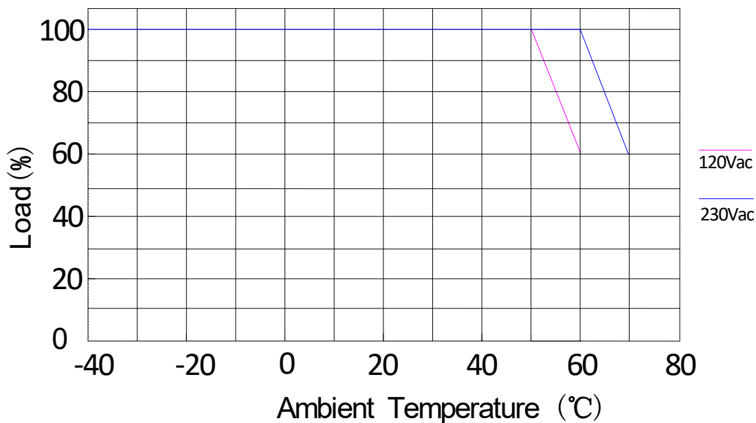
Derating Curve
