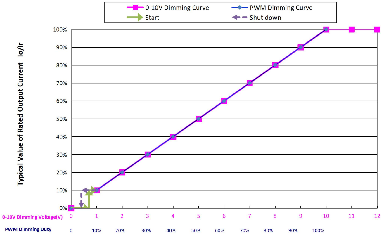
0-10V/PWM Dimming Curve
