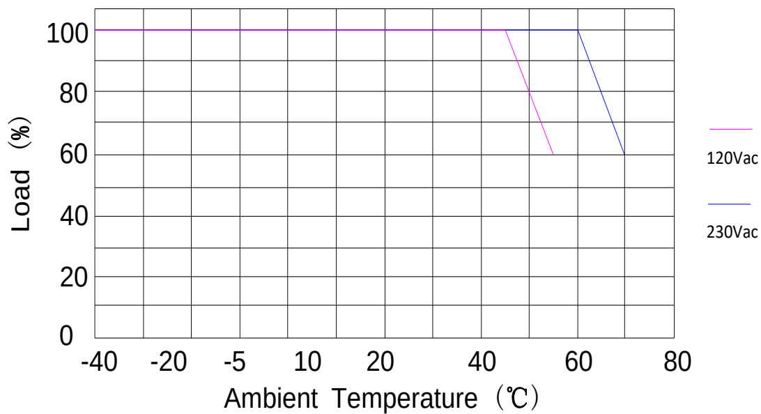
Derating Curve
