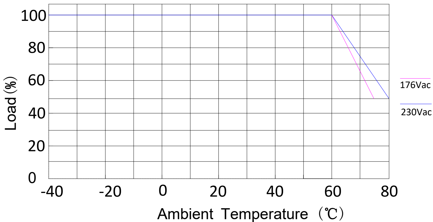
Derating Curve
