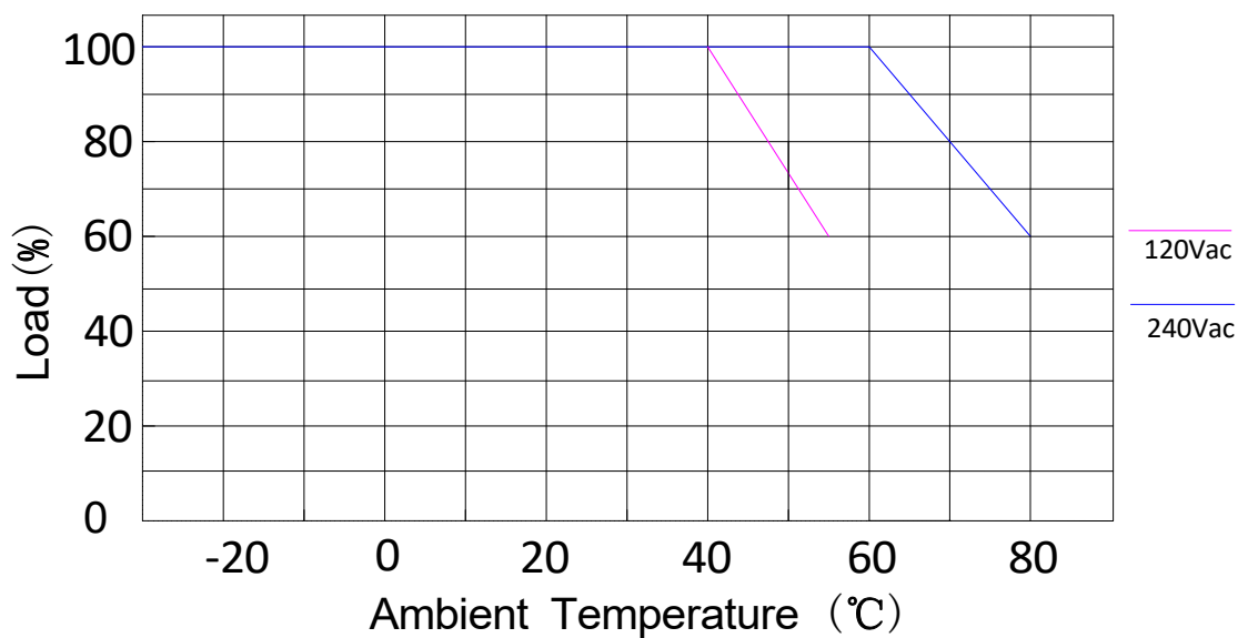
Derating Curve
