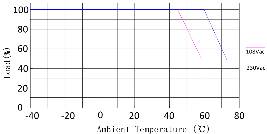
Derating curve
