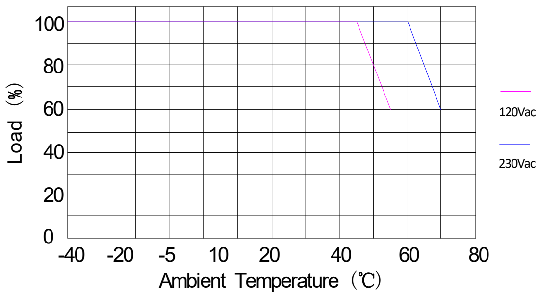
Derating Curve
