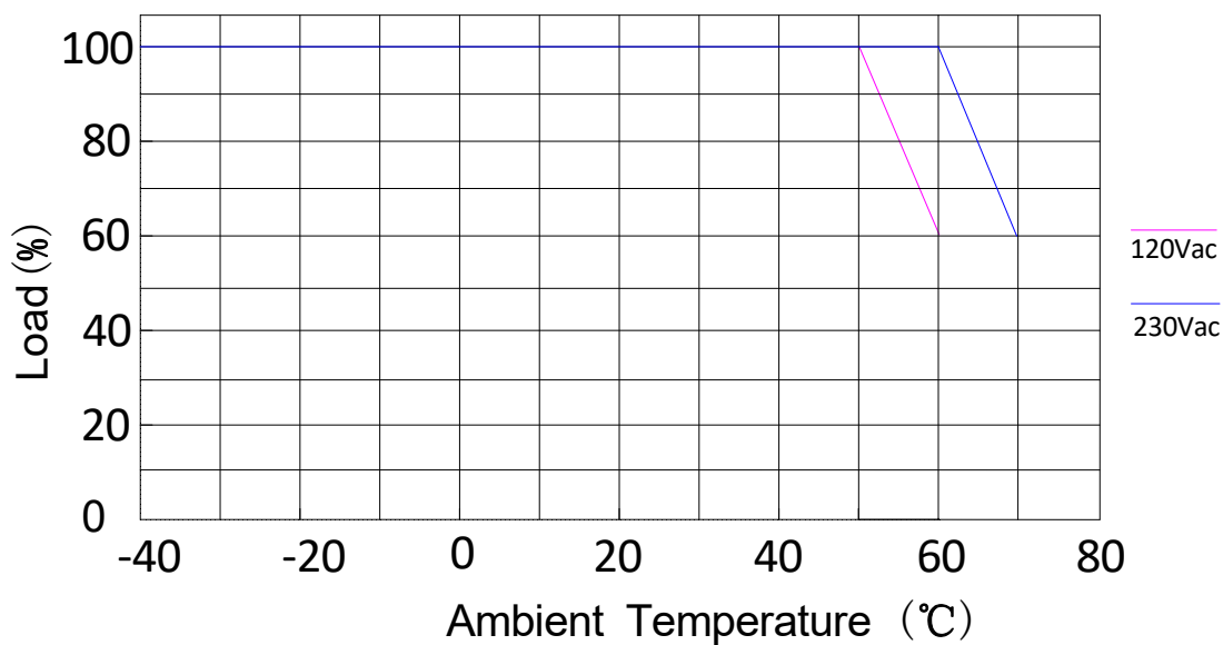
Derating Curve
