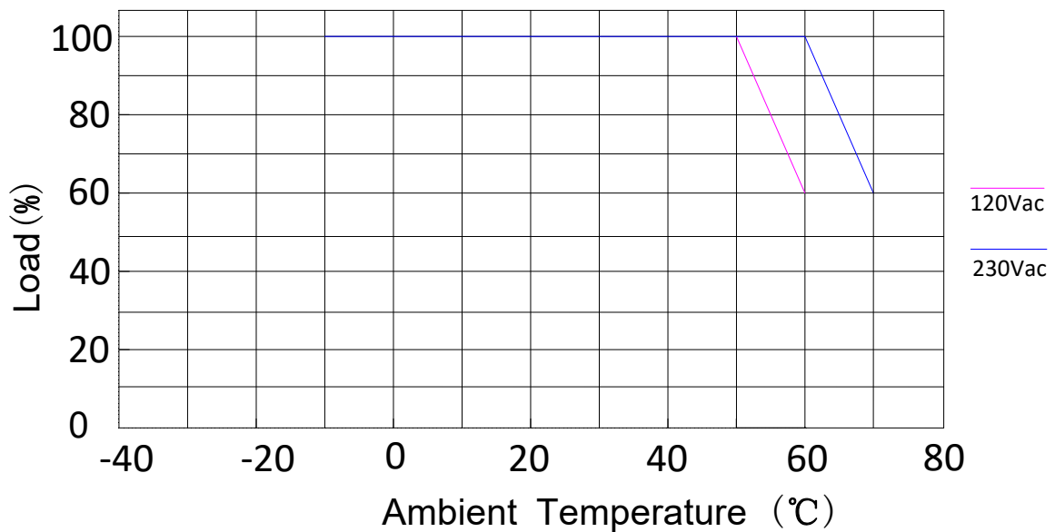
Derating Curve
