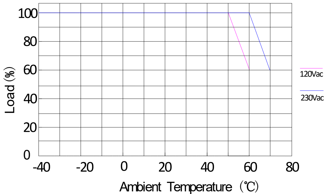
Derating Curve
